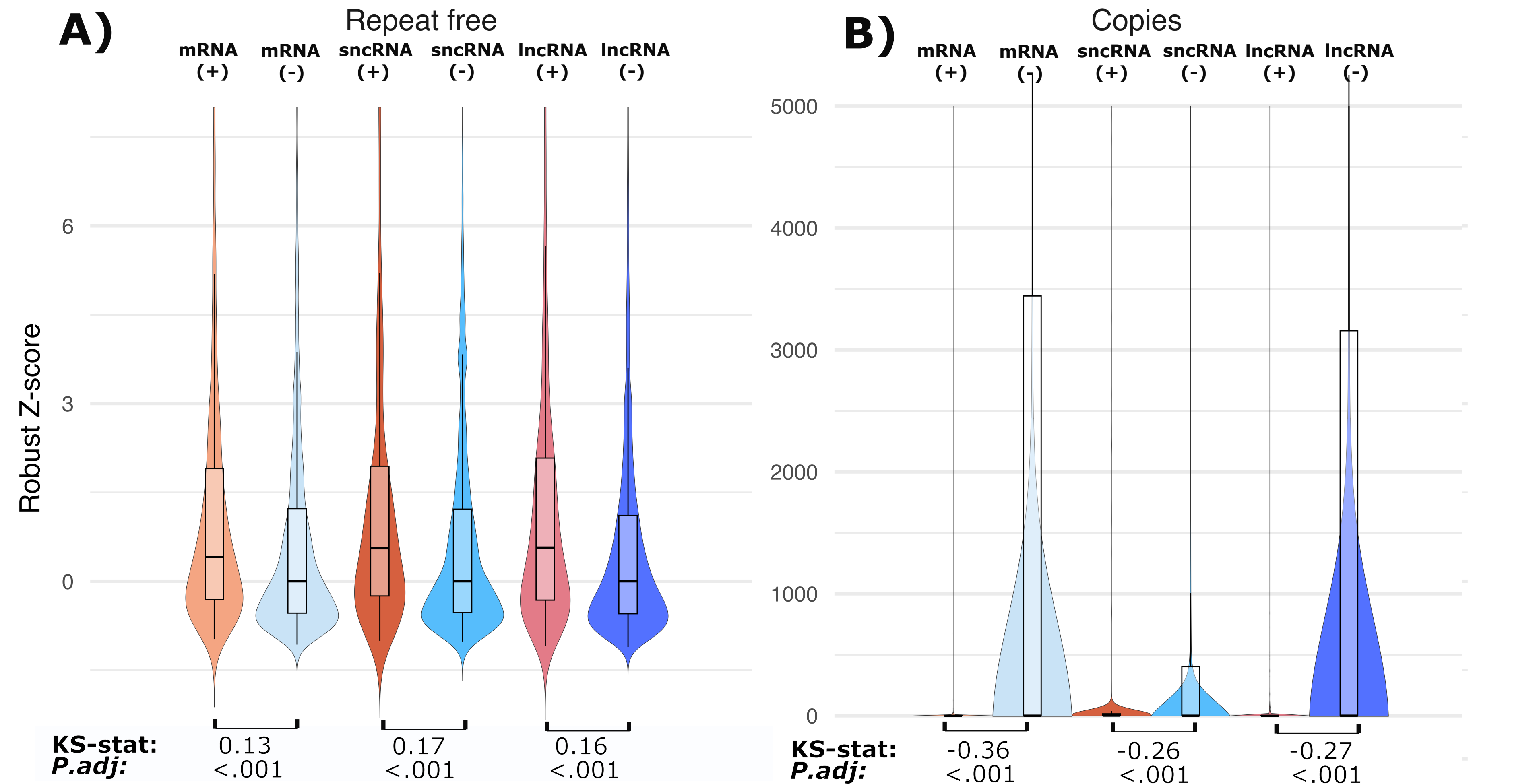
Figure 6. Violin plot and box plots for the distribution of repeat association features based on robust z-scores for genic and matched non-genic regions. A) Repeat free, combined distance to nearest up and downstream repeat elements (SINE, LINE, etc) that does not overlap each control sequence. B) Copies is the genomic copy number of each analyzed region as determined by MMseqs2 searches of the GRCh38 genome. Signed Kolmogorov-Smirnov statistics and adjusted p-values are displayed under each comparison.
